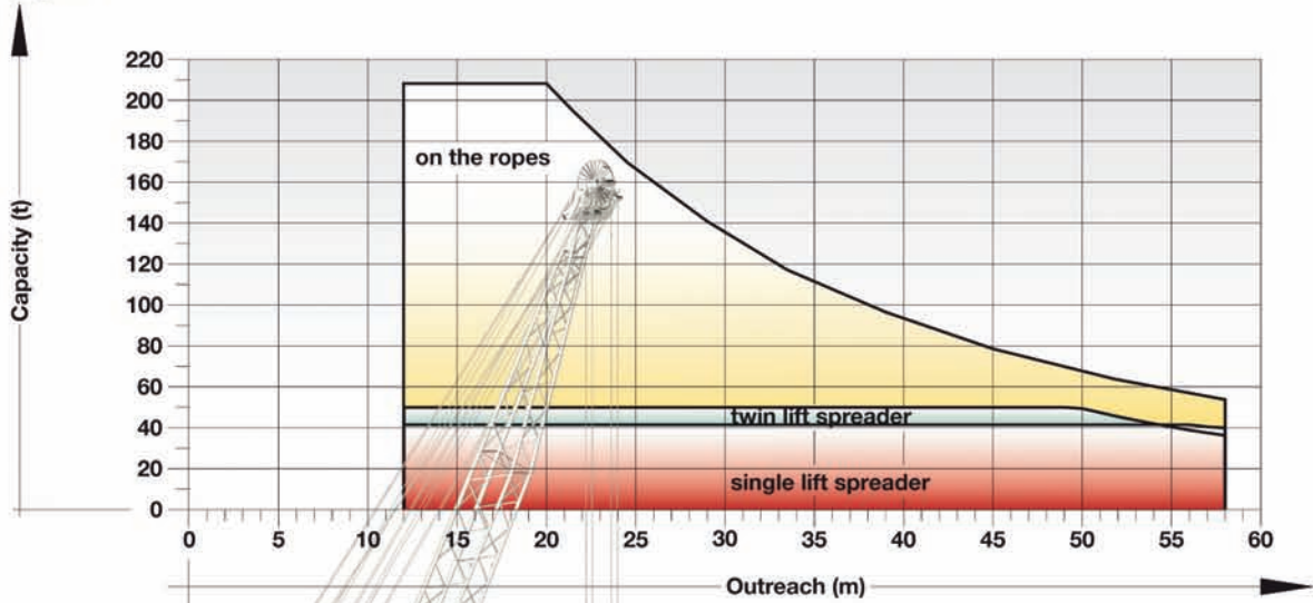
Load diagram
